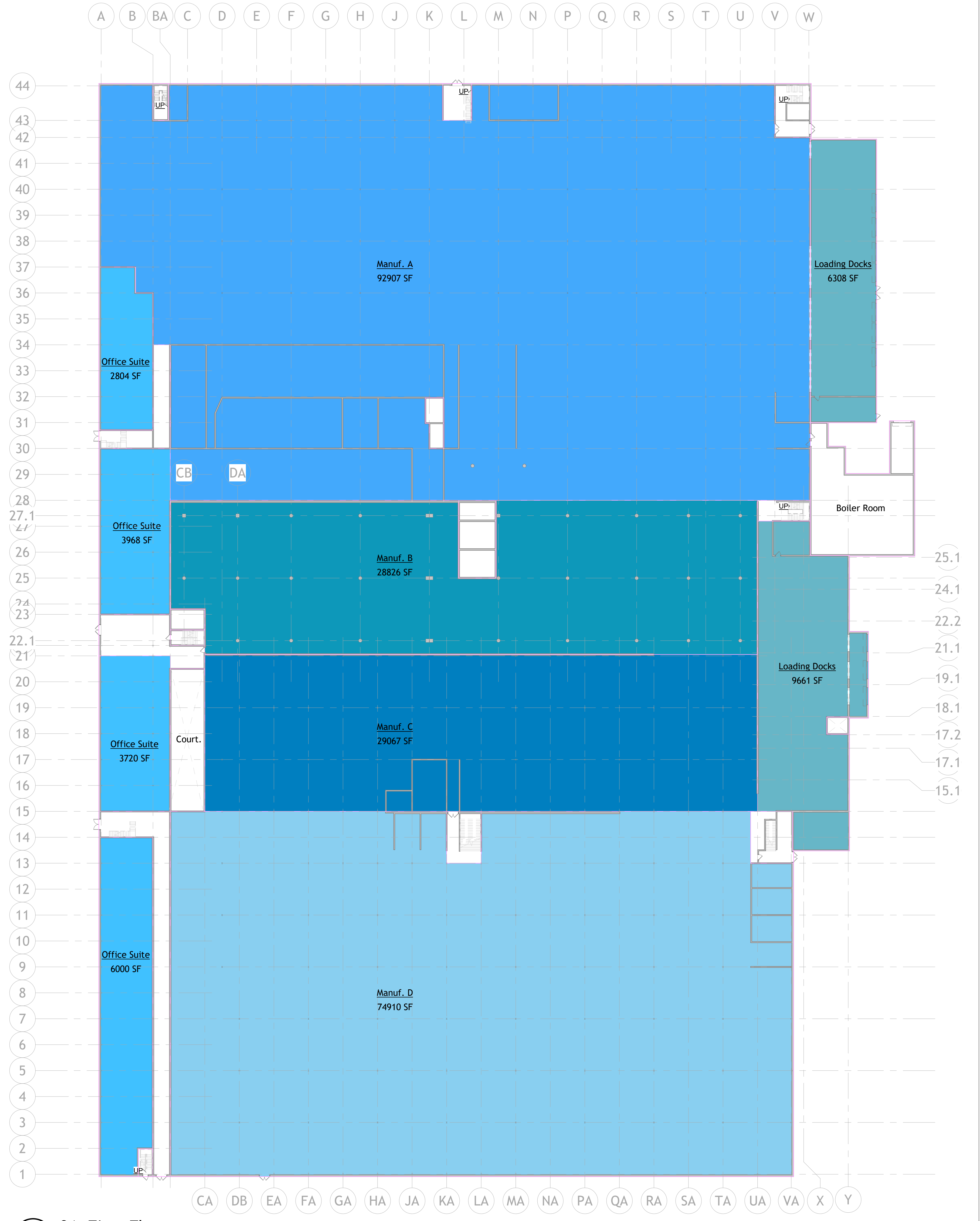
1 01_First Floor 1" = 30'-0"
